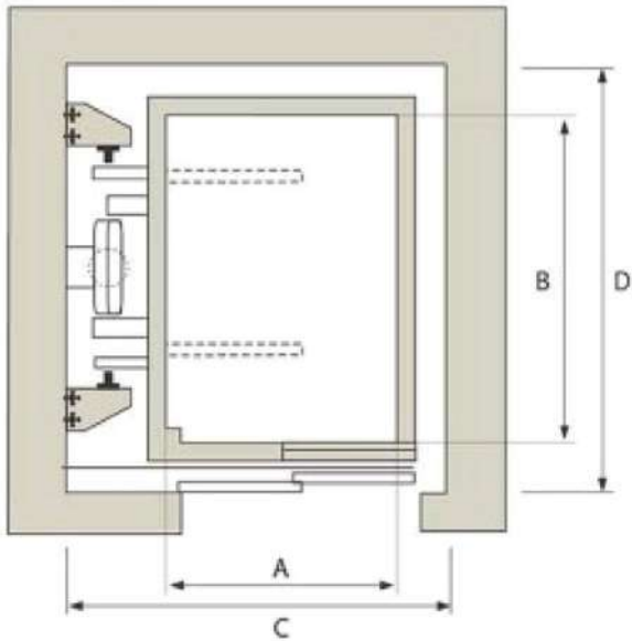
Hoistway Elevation & Plan
